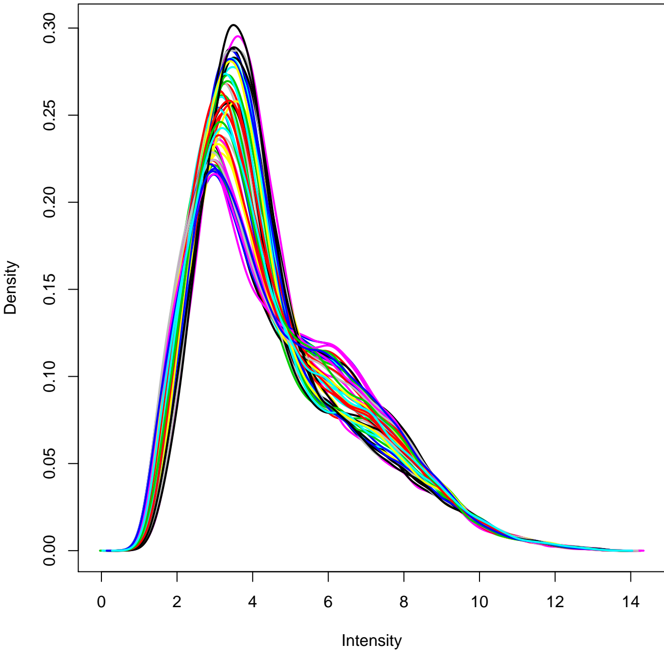
GSE57214/GPL17400 value distribution
